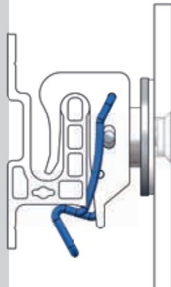
Hook system with anti-lift clip
