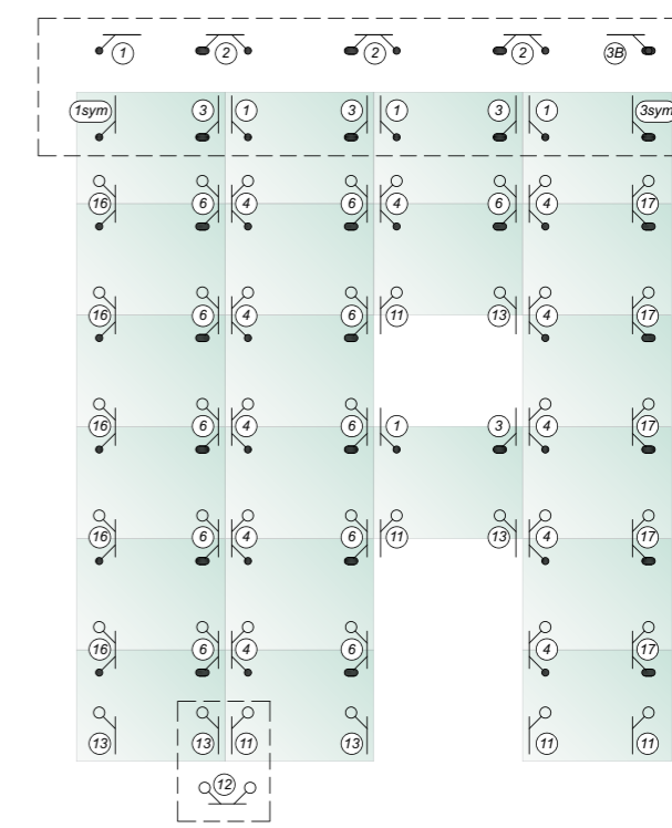
Mounting - F
